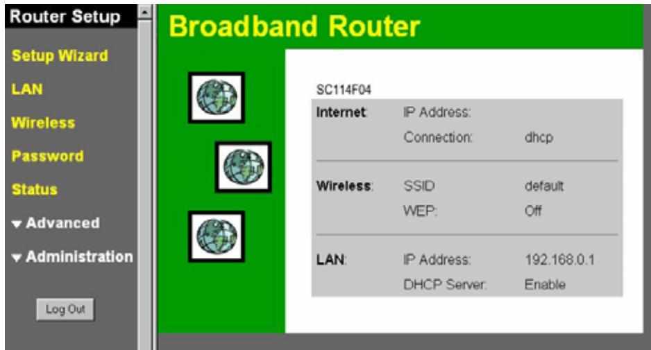
Figure 5: Home Screen
