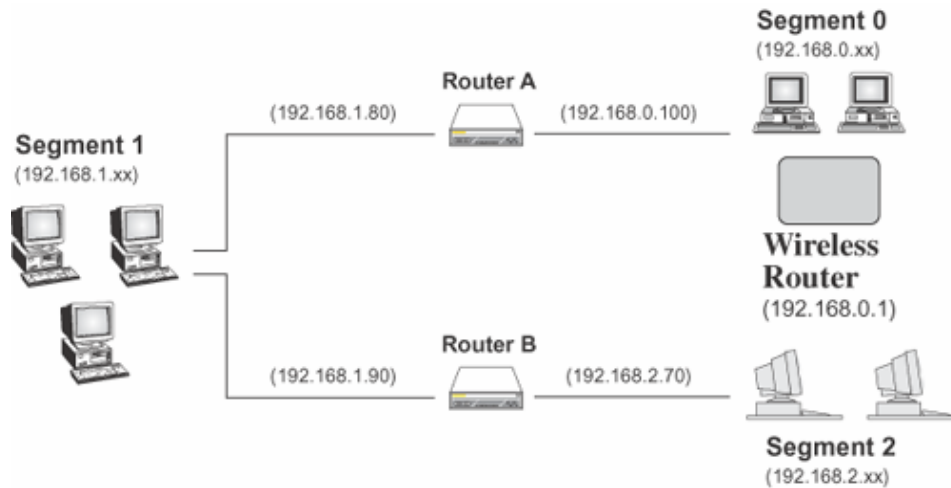
Figure 49: Routing Example
