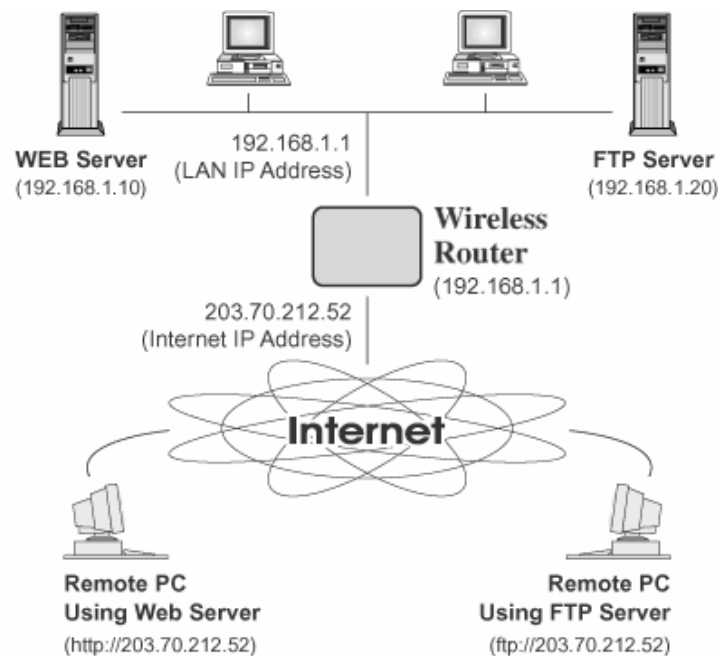
Figure 38: Virtual Servers
