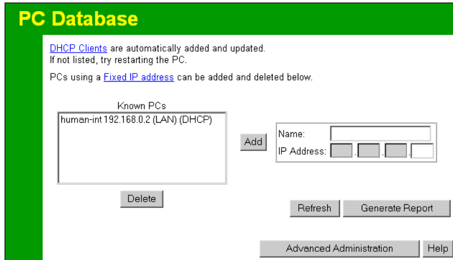
Figure 45: PC Database
