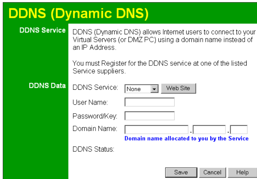
Figure 34: DDNS Screen
