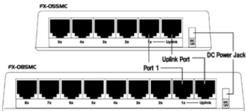
FX-05SMC/08SMC Rear View
